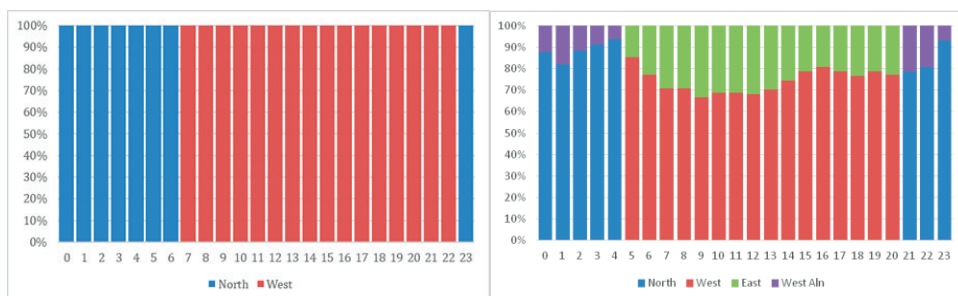
Figure 4: Daily distribution of Planned and Actual Runway configuration, selected days in summer 2019
