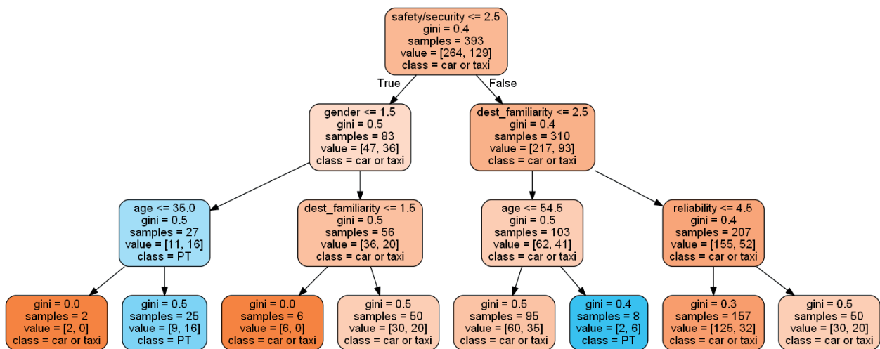
Figure 4: Decision tree for classification airport access mode choice in two classes: PT and car or taxi
